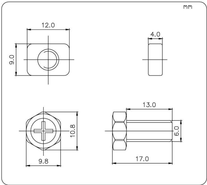
Screw
