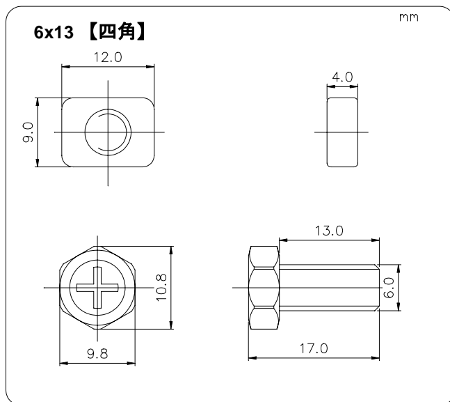
Screw
