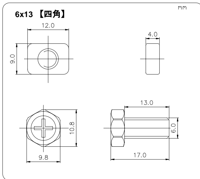
Screw
