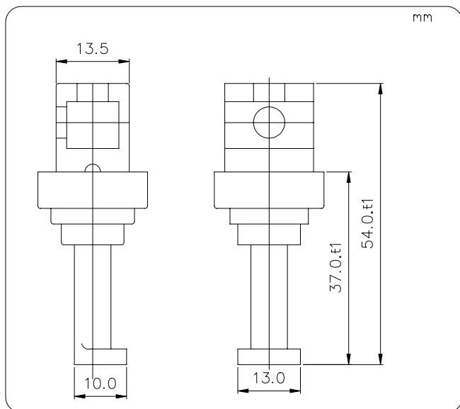
Terminal
