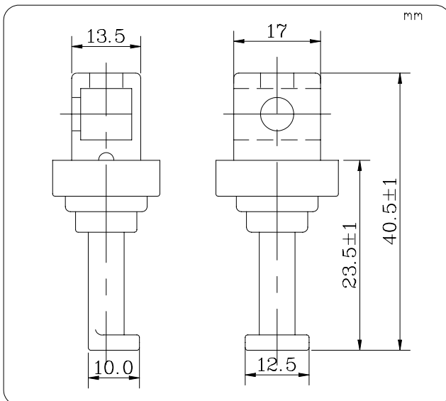
Terminal
