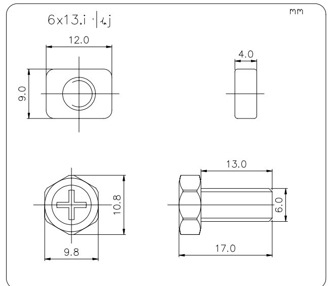
Screw
